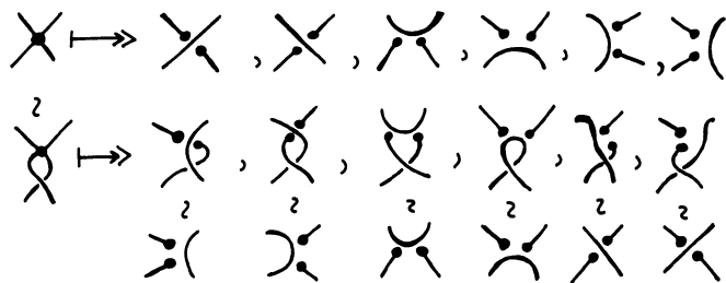
FIGURE 7. Braiding at a vertex permutes the replacements
