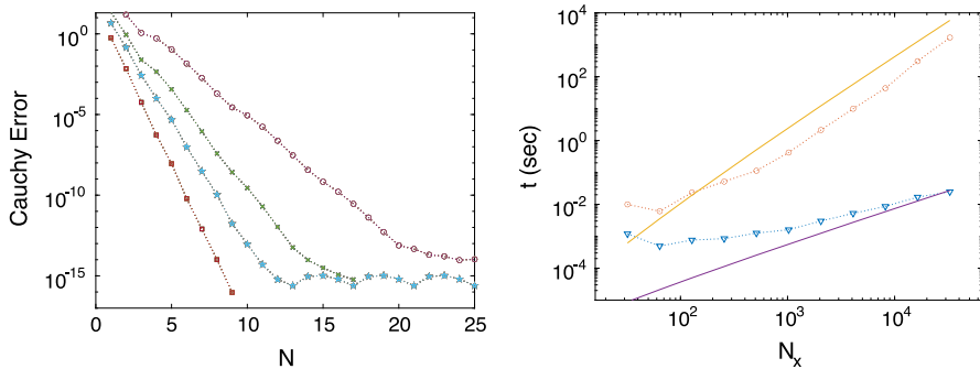
Fig. 2 Left: The Cauchy error, (18), measured for a Wilton ripple in each of the PDEs listed in Table 1 from the FPI (14) at \varepsilon = 0.01 . The markers correspond to the PDEs as follows: (A) circles, (B) xs, (C) stars, (D) squares. Right: The run times for our novel FPI (triangles) and the quasi-Newton method (circles) as a function of the number of spatial points. The amplitude parameter \varepsilon = 0.01 was simulated for the Akers–Milewski equation. The asymptotic curves N_x^2 \log N_x and N_x \log N_x are plotted with solid lines
