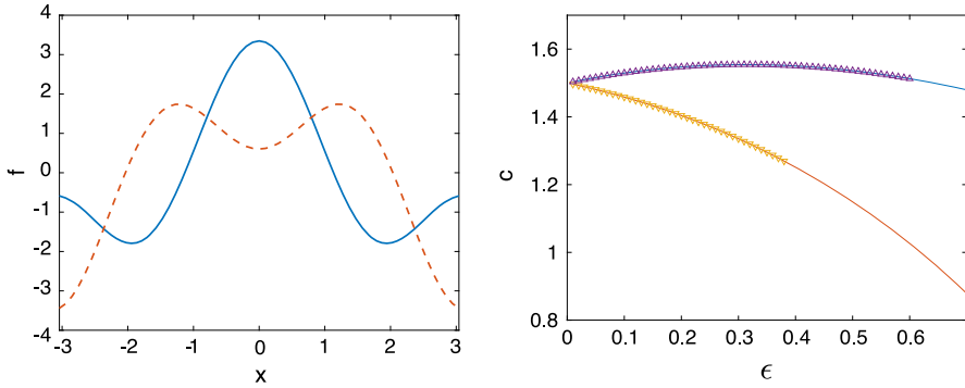
Fig. 1 Left: Example profiles from the FPI, (14), with \varepsilon = 0.01 (the profile on branch with \beta = 1/\sqrt{2} , (12), is the solid curve, the profile on the branch with \beta = -1/\sqrt{2} is the dashed curve). Right: The speed–amplitude curves for two branches of ripples in the Akers–Milewski equation are depicted. The output of the FPI (triangles) is compared to that of the quasi-Newton iteration (solid lines)
