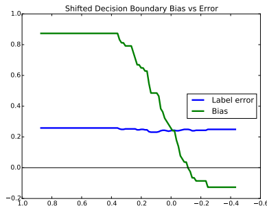
(a) Boosting
