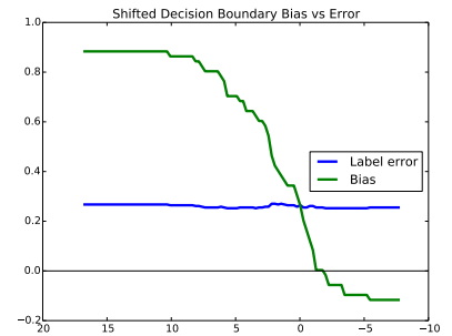
(c) SVM
