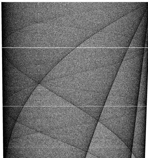
Figure 5. Blowup near c = -2 .
