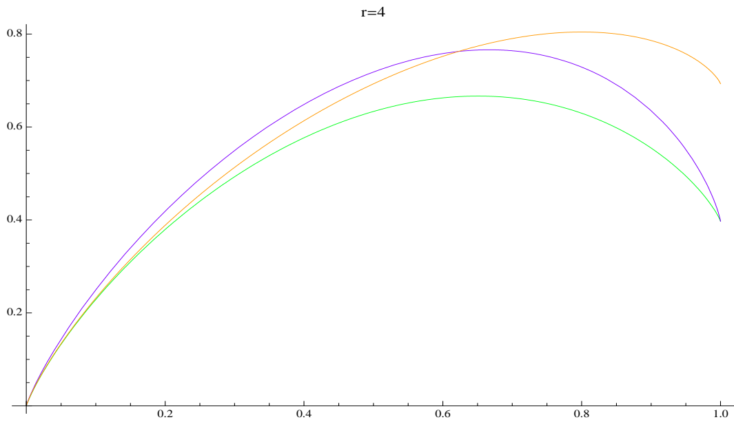
Figure 3: h_{K(4)} -green, upp_{4,1} -blue, upp_{4,2} -orange, color online
