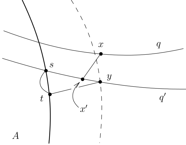
FIGURE 7. Tube lemma.
