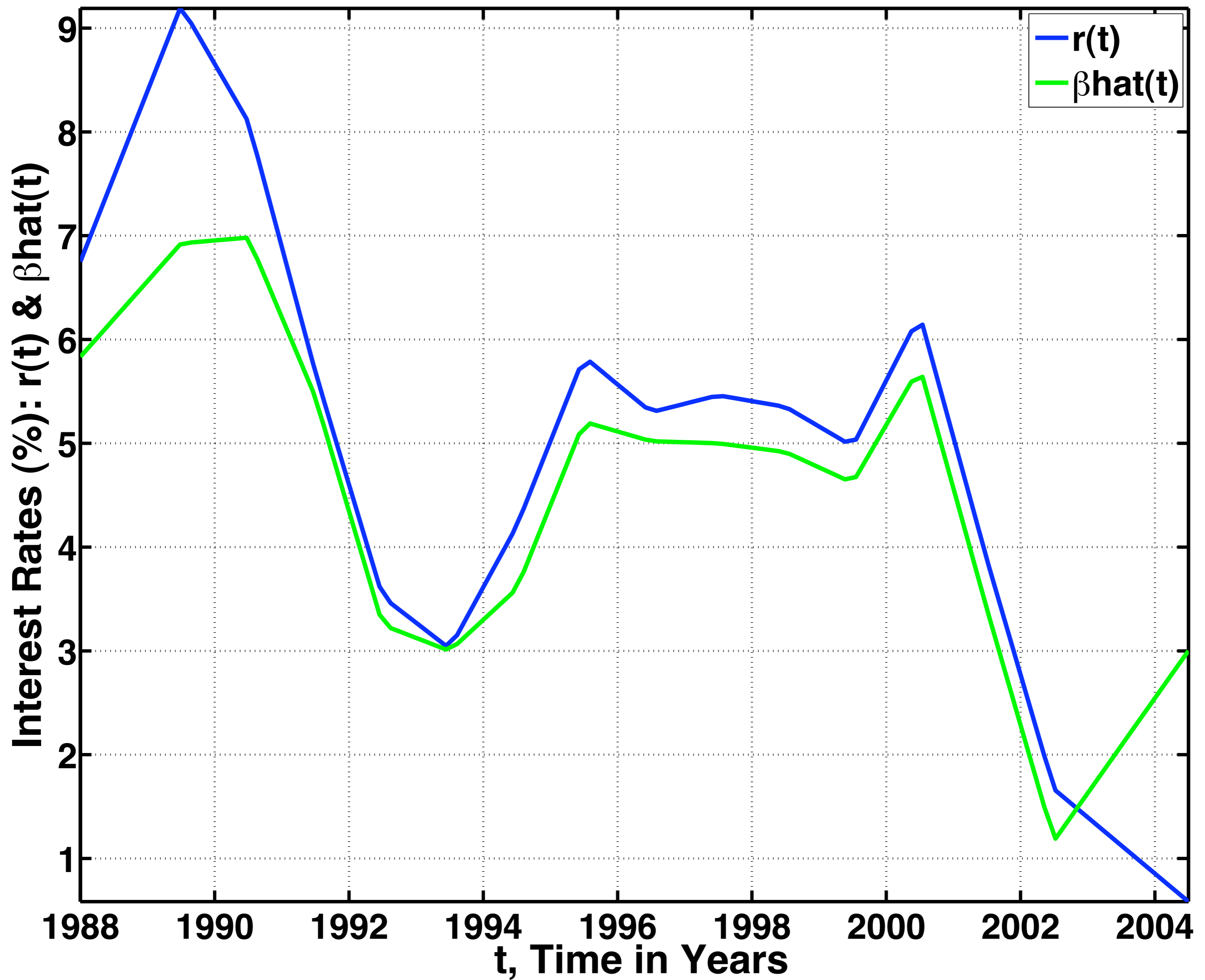
Federal Funds Rates (%) r(t) & \hat{\beta}(t) versus t
