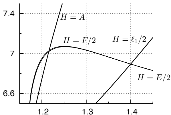
FIGURE 3.1. The volume estimates of Kojima–Miyamoto
