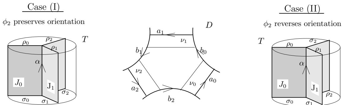
FIGURE 5.2. Some objects defined in the proof of Lemma 5.9
