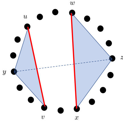
Figure 7: Edge \{y, z\} absent from \partial H
