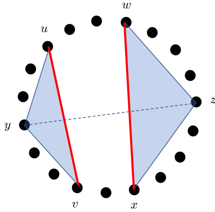
Figure 7: Edge \{y, z\} absent from \partial H
