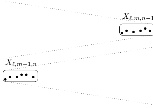
Figure 1: Construction for X_{\ell, m, n} from X_{\ell, m, n-1} and X_{\ell, m-1, n} .
