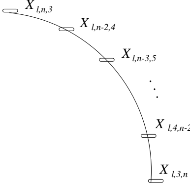
Figure 2: The lower bound construction for ES_\ell(n) .
