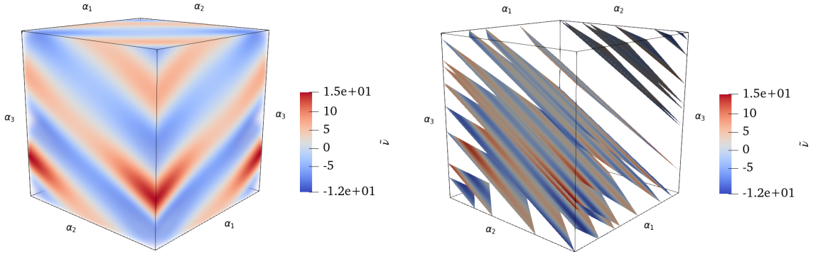
Figure 5: Plot of the computed Neumann data, \tilde{u} , for \varepsilon = 0.16 . (a) The full field; (b) A slice of the full field with a plane that has normal vector (1/\sqrt{2}, -1/\sqrt{3}, -1)^T .
