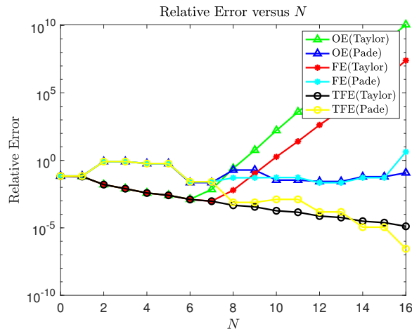
Figure 2: Plot of relative error, (6.4), for a medium perturbation ( \varepsilon = 0.5 ) in the surface Neumann data for the three HOPS algorithms (OE, FE, TFE) using both Taylor and Padé summation. Physical parameters were (6.2) and numerical discretization was (6.3).
