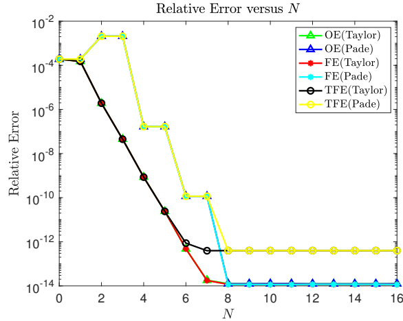
Figure 1: Plot of relative error, (6.4), for a small perturbation ( \varepsilon = 0.02 ) in the surface Neumann data for the three HOPS algorithms (OE, FE, TFE) using both Taylor and Padé summation. Physical parameters were (6.2) and numerical discretization was (6.3).
