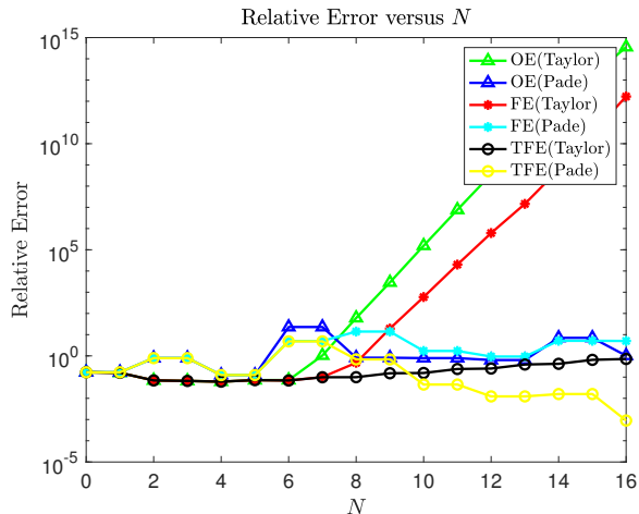
Figure 3: Plot of relative error, (6.4), for a large perturbation ( \varepsilon = 1 ) in the surface Neumann data for the three HOPS algorithms (OE, FE, TFE) using both Taylor and Padé summation. Physical parameters were (6.2) and numerical discretization was (6.3).
