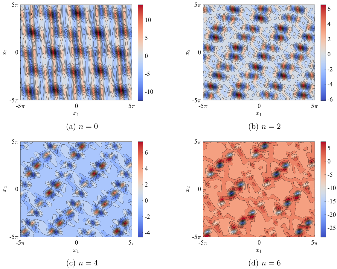
Figure 6: Contour plots of the Taylor corrections \tilde{v}_n for n = 0 (panel (a)), n = 2 (panel (b)), n = 4 (panel (c)), and n = 6 (panel (d)).
