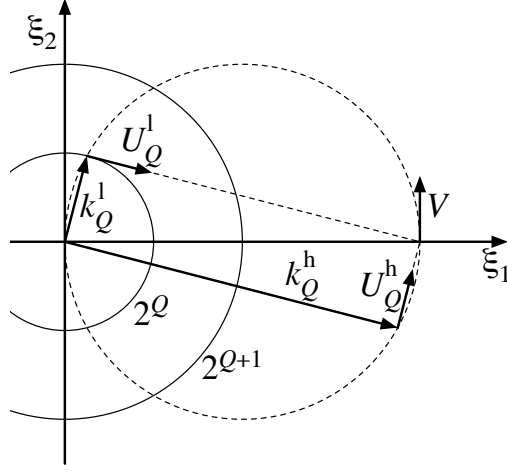
FIGURE 1. Construction of the vector field illustrating infrared nonlocality.
