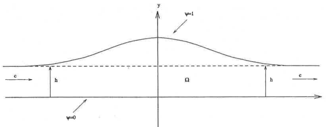
Fig. 1. The solitary wave.
