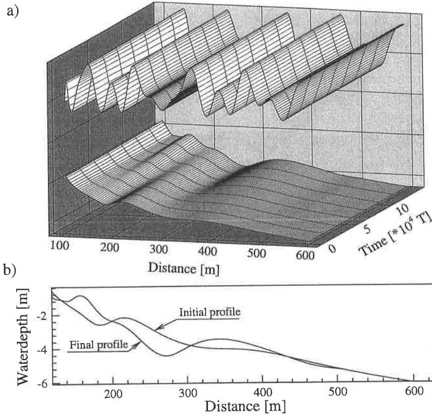
Figure 10: Prediction of an episodic change in the two-bar system at Duck, NC (a) migration of the post-storm profile under extreme waves ( T_p = 15 s), accompanied by a 1.2-m surge above the mean water level, (b) initial and final bed profiles from (a).
