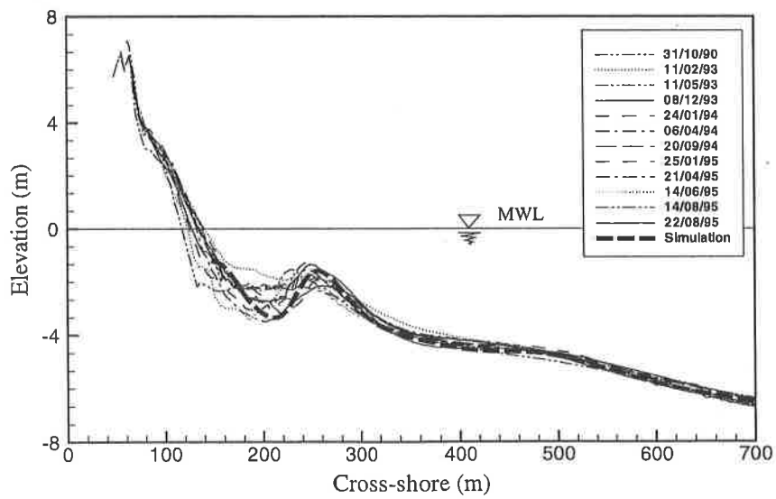
Figure 8: Comparison of predictions (heavy dashed line) and measurements of an observed two-bar system at Duck, NC (with bar crest positions at 250 m and 500 m).
