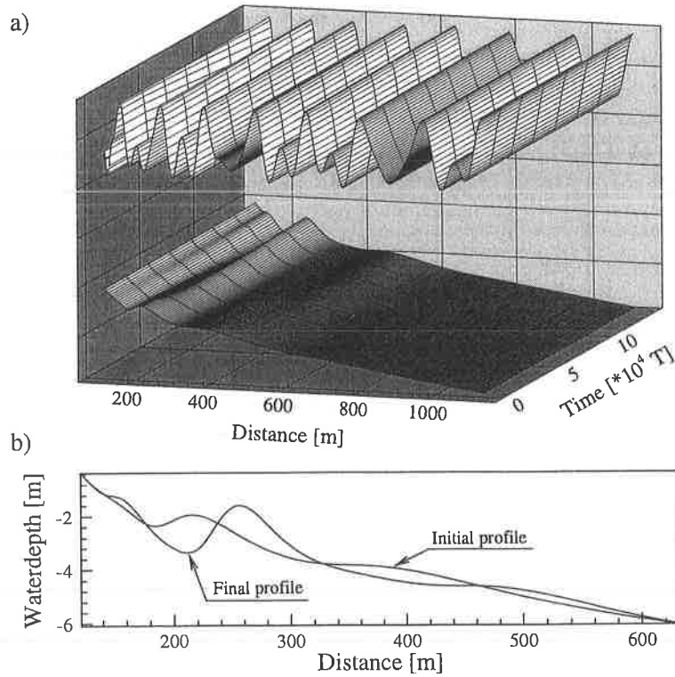
Figure 6: Prediction of changes from the typical two-bar system by extreme autumn-winter storms (with T_p = 17.5s ): (a) temporal evolution of the new two-bar system from the original two-bar profile, (b) initial and final profiles from (a).
