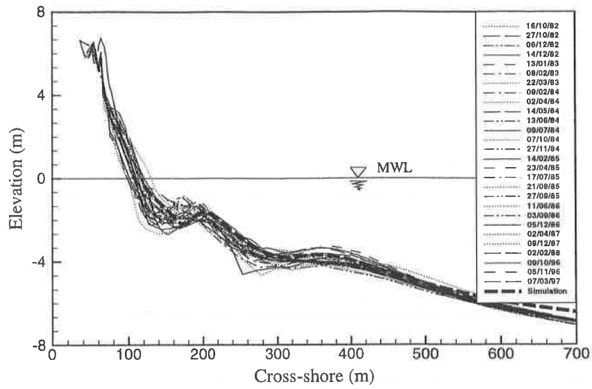
Figure 5: Comparison of predictions (heavy dashed line) and measurements of the most frequently-observed two-bar system at Duck, NC
