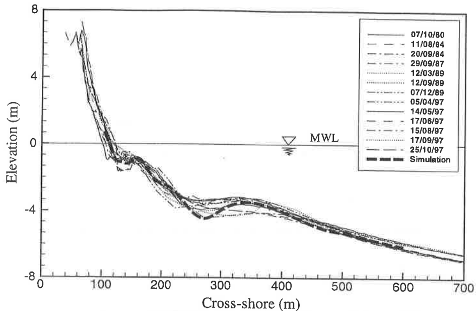
Figure 11: Prediction (heavy dashed line) and observations of episodic, nonstationary behavior of the two-bar system at Duck, NC.
