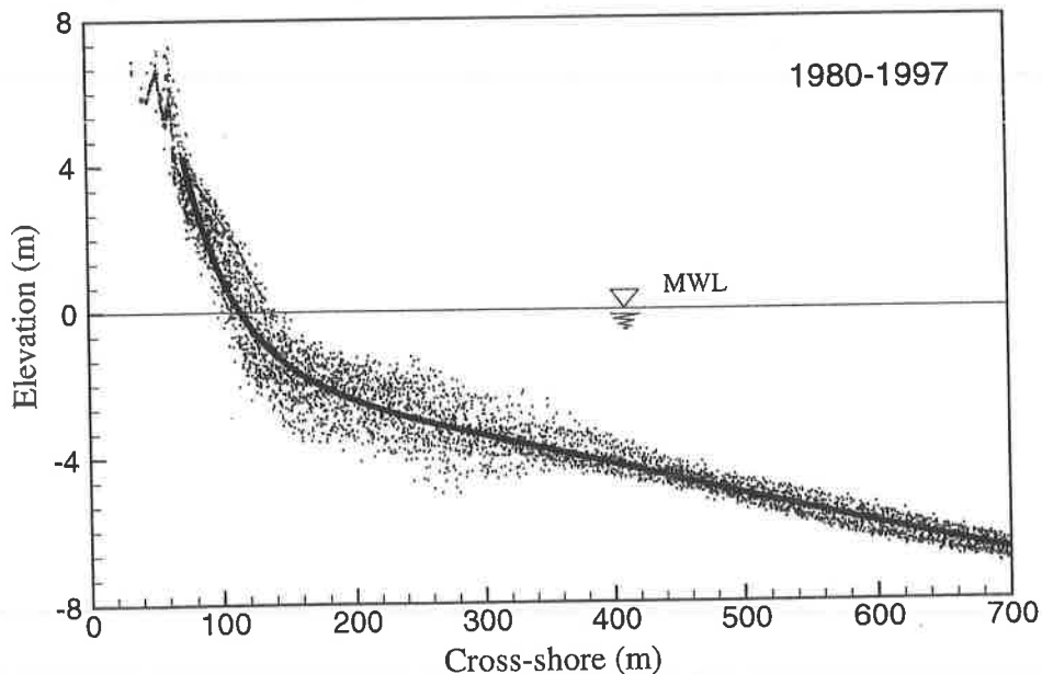
Figure 1: Foreshore morphology data at profile 62, Duck, NC, (1980-1997) and the featureless equilibrium profile
