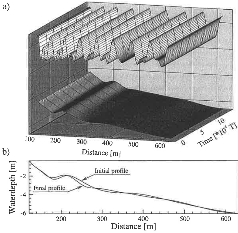
Figure 7: Prediction of changes from the typical two-bar system by moderate summer storms (with T_p = 10s ): (a) temporal evolution to a one-bar system from the typical two-bar profile, (b) initial and final profiles from (a).
