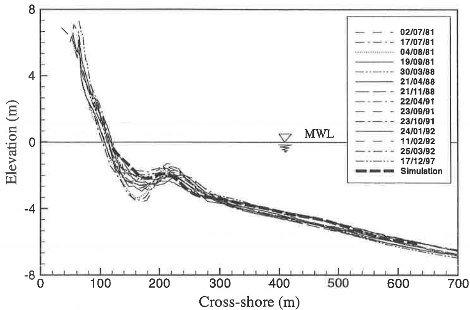
Figure 9: Comparison of predictions (heavy dashed line) and measurements of an observed one-bar system at Duck, NC (with the bar crest position at 220 m).
