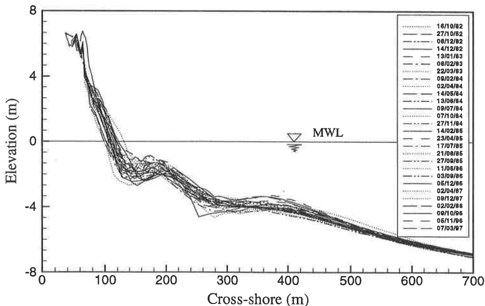
Figure 2: Typical two-bar system at Duck, NC, with indicated dates of data acquisition (based on measurements at cross-section 62)
