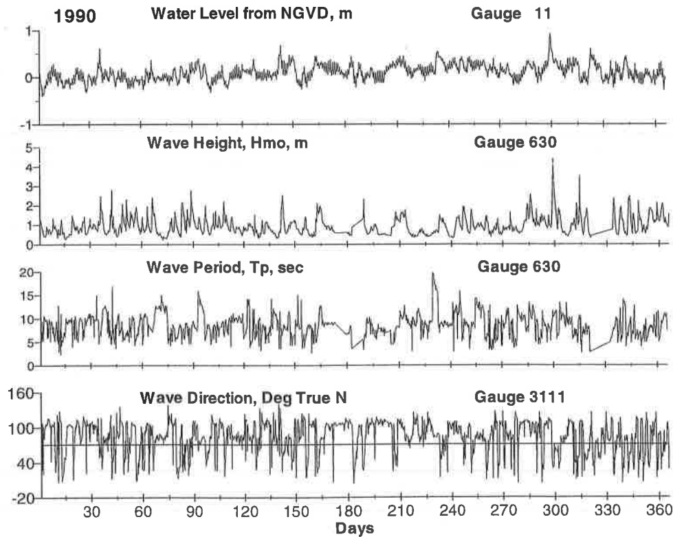
Figure 3: Observed wave and water level parameters at Duck, NC, in 1990
