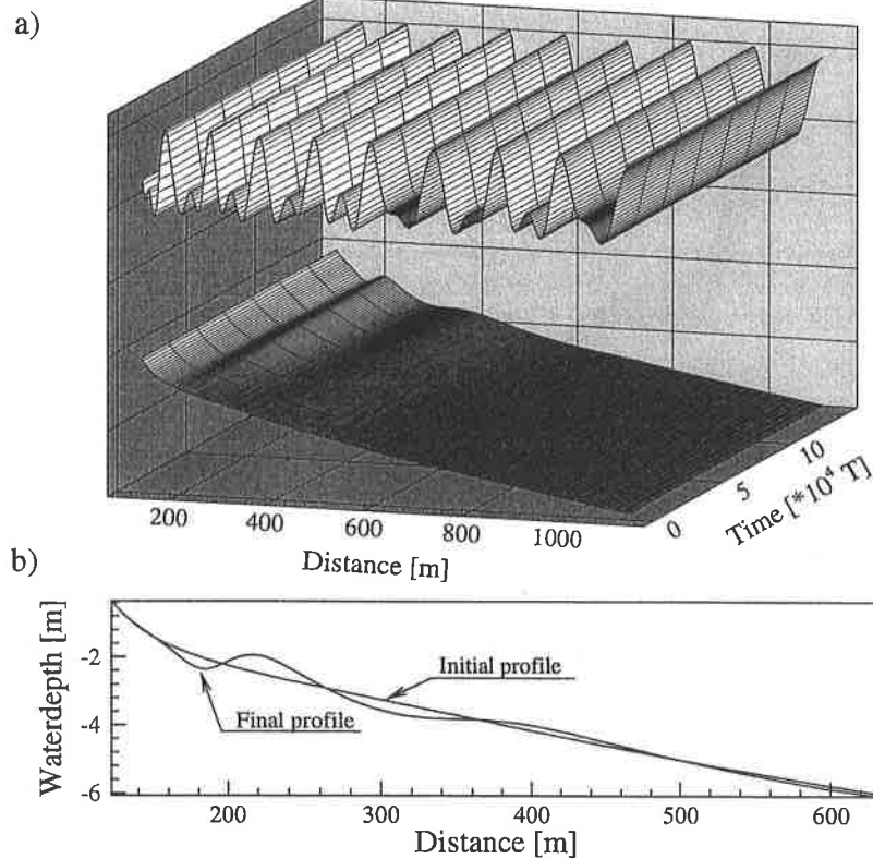
Figure 4: Prediction of the formation of the typical two-bar system by major storms (with T_p = 15 s) at Duck, NC: (a) temporal evolution of the bar system from the featureless equilibrium profile, (b) initial and final profiles from (a).
