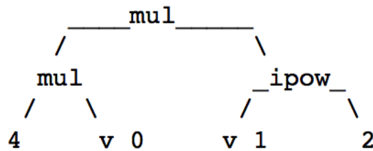
Fig. 1.10: The binary expression tree of 4*x*y^2 .
