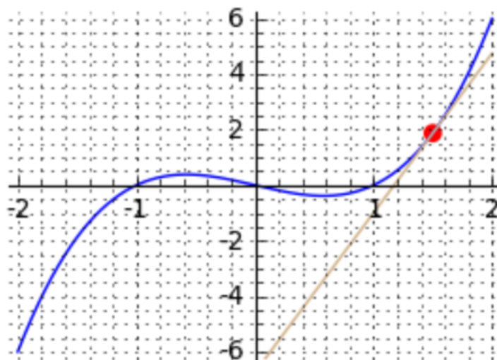
Fig. 5.2: The tangent line of x^3 - x for x = 1.5 .
