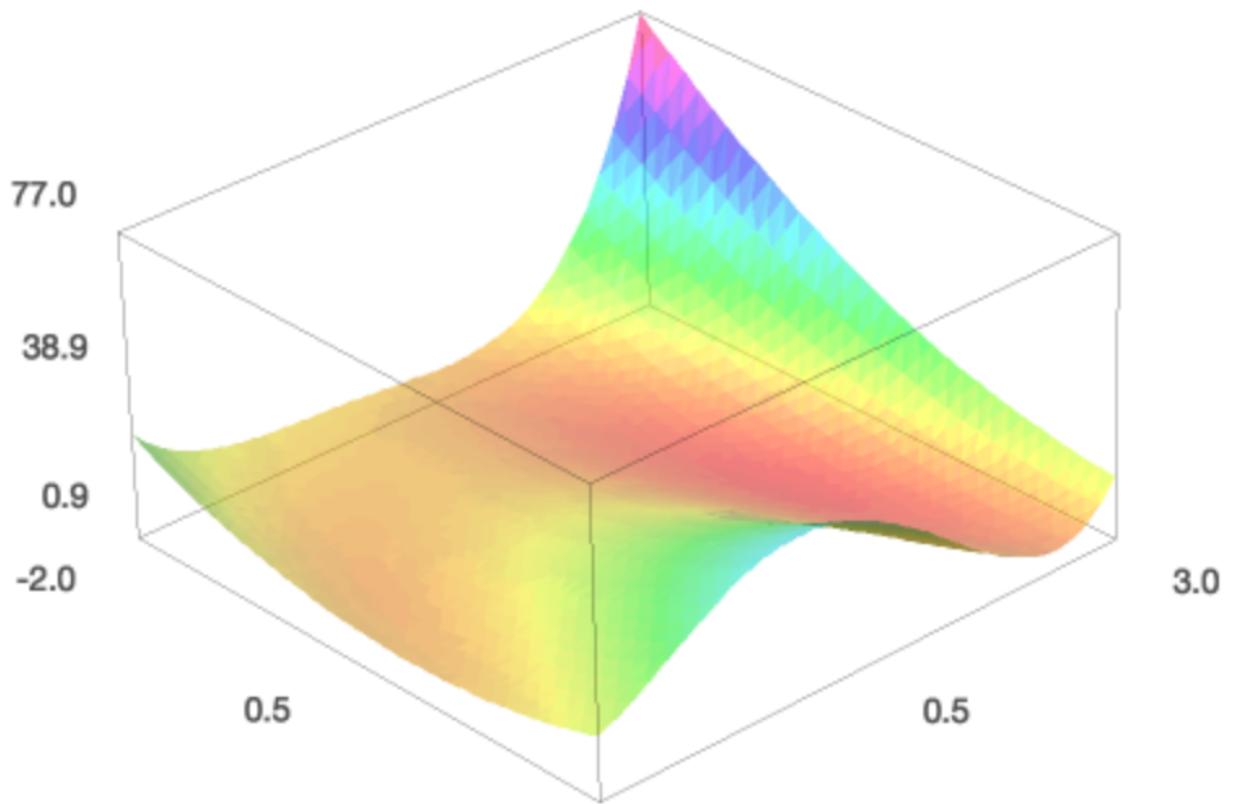
Fig. 4.47: Looking for the location with the smallest height on a surface.
