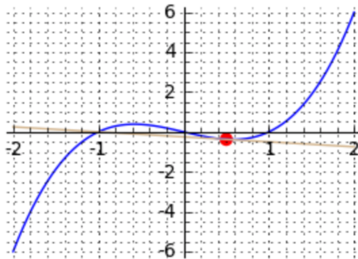
Fig. 5.1: The tangent line of x^3 - x for x = 0.5 .
