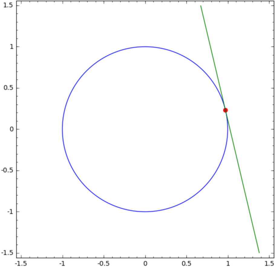
Fig. 3.7: The tangent line to a point on a circle.
