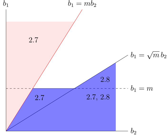
Figure 2-2: Theorems 2.2.7 and 2.2.8 for \vec{\mathbf{b}} = (b_1, b_2, 1)
