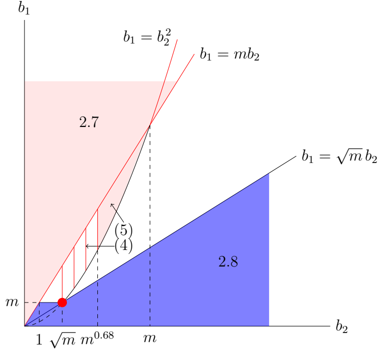
Figure 2-3: \vec{b} = (b_1, b_2, 1)
