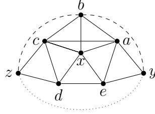
Figure B-8: Case 2: y \neq z , ae y and cdz are triangles in H .
